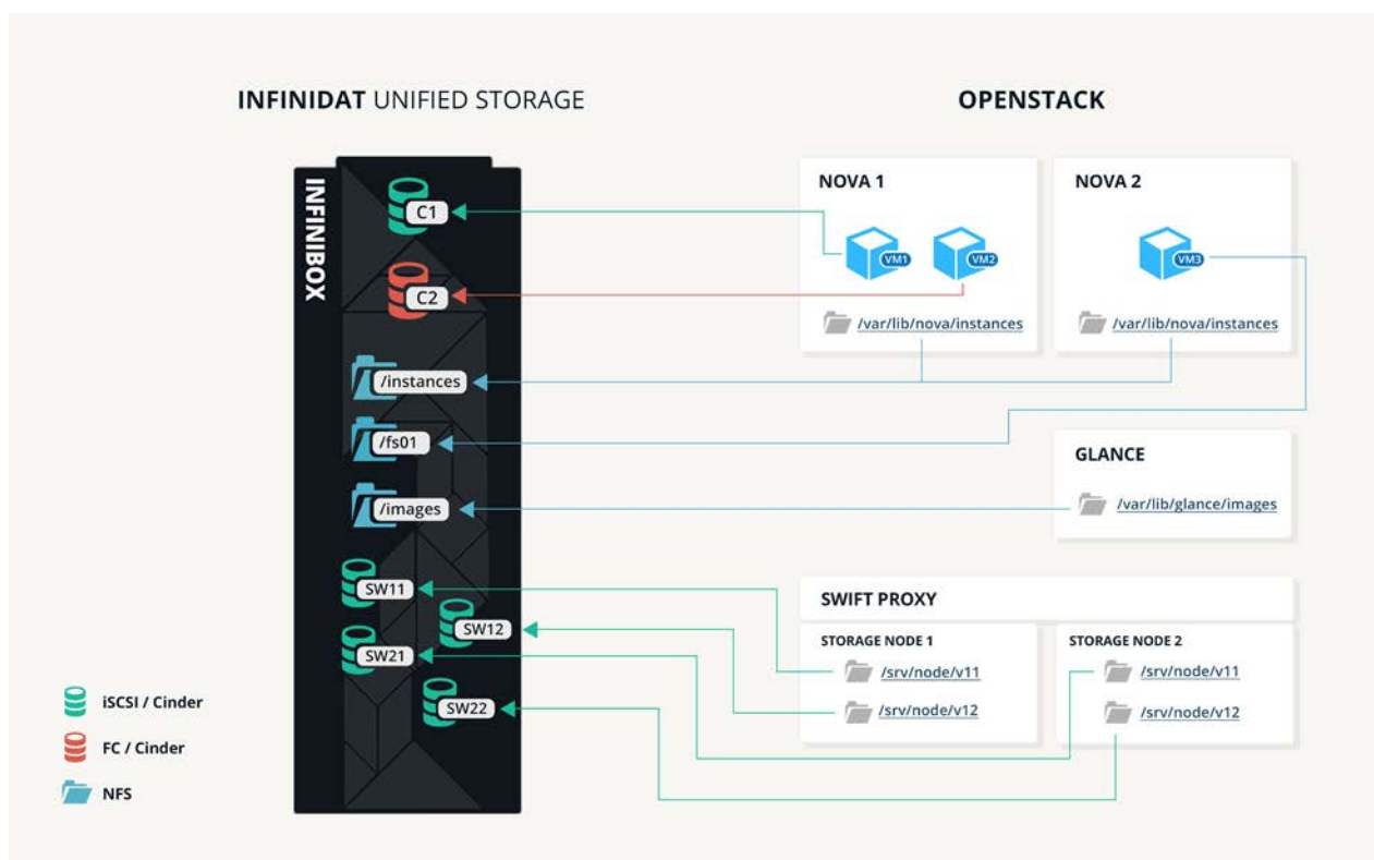
INFINIDAT Unified Storage Catering to all OpenStack Storage Needs
